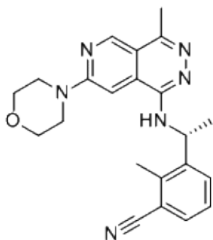
PC-73313, DMSO-d6
